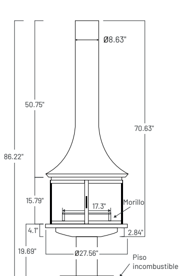
Vista frontal
