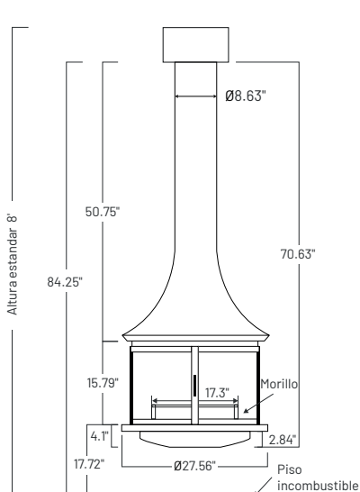
Vista frontal
