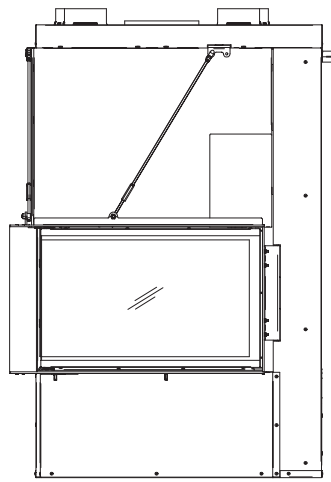
Vista frontal
