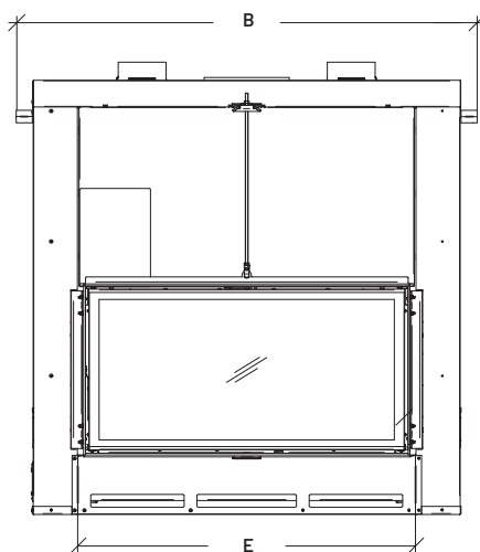
Vista frontal
